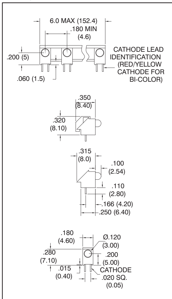
3mm PC Board Mount LED
