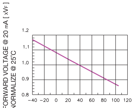
AMBIENT TEMPERATURE T_a (°C) FORWARD VOLTAGE VS. TEMPERATURE
