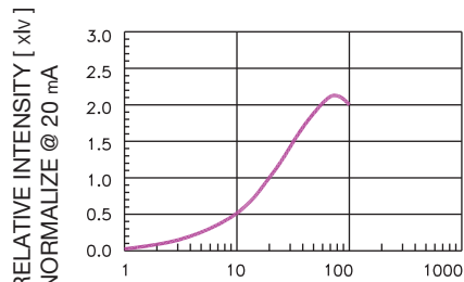
RELATIVE INTENSITY [xlv] NORMALIZE @ 20 mA FORWARD CURRENT I_F (mA) RELATIVE INTENSITY VS. FORWARD CURRENT
